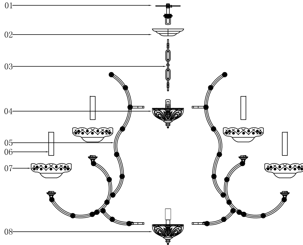
lamp body(04)parts list
